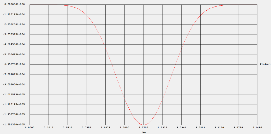
Associated Legendre Function l = 7 m = 7
